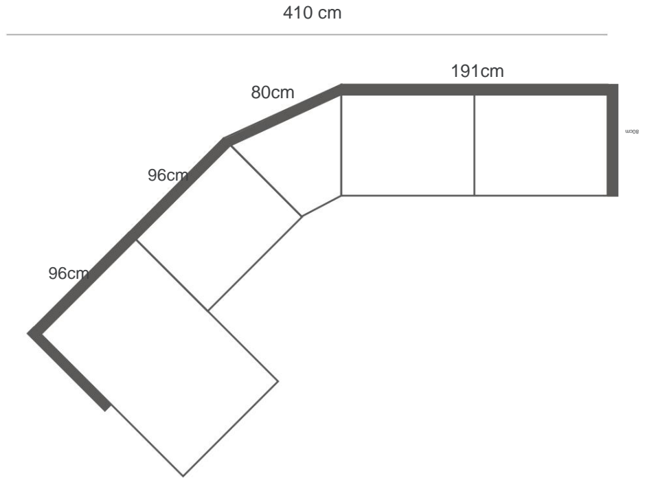
DRAWING 6 1 x 96 cm chaise longue w / A arm left 1 x 1.5 seat module w / out arms 1 x 45° corner module 1 x 3 seat module 2 cushions w / A arm right
